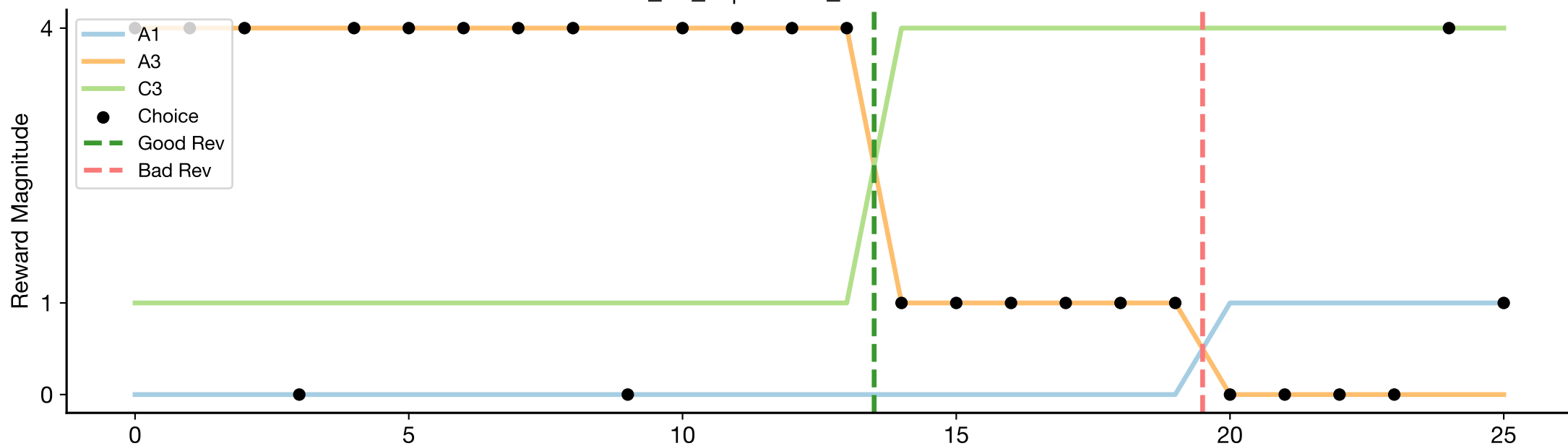
RT_64_R | ses-26_date-20260925
